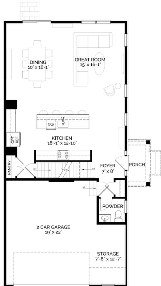
MAIN FLOOR
