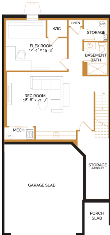
BASEMENT
